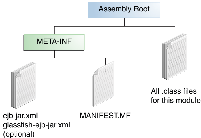
FIGURE 22-2 Structure of an Enterprise Bean JAR
