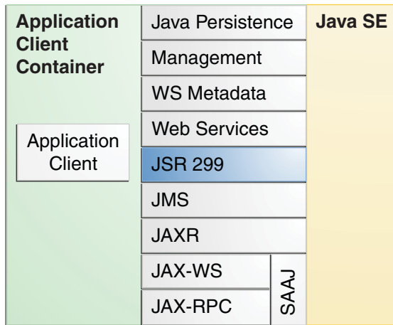
FIGURE 1-10 Java EE APIs in the Application Client Container
