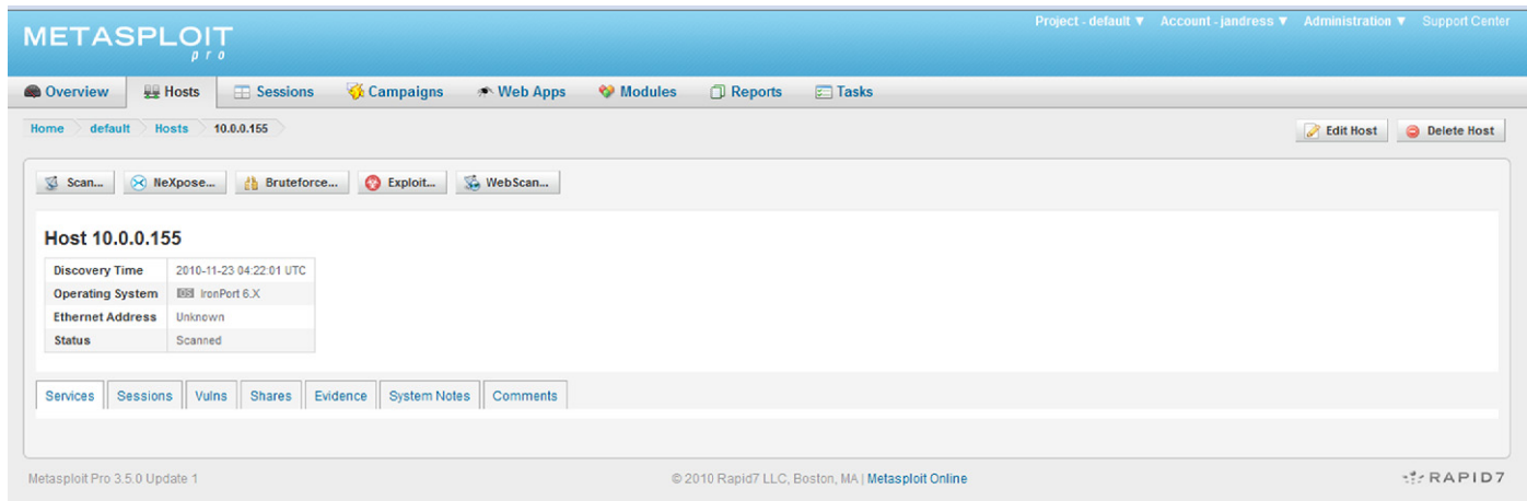
FIGURE 6.15 Metasploit Pro.
