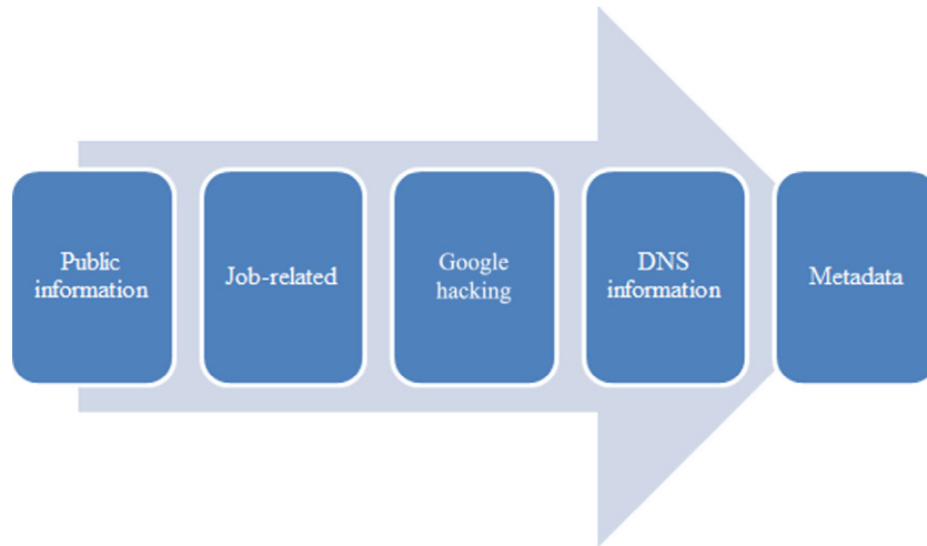
FIGURE 9.1 OSINT process.
