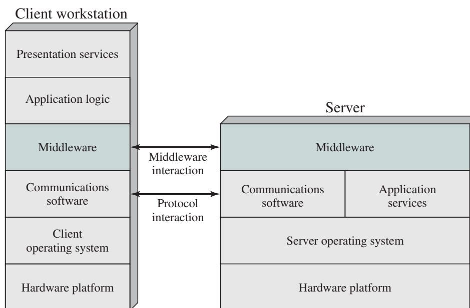
Figure 16.8 The Role of Middleware in Client/Server Architecture
