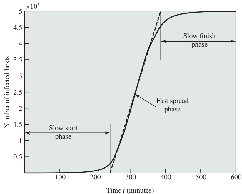
Figure 14.5 Worm Propagation Model
