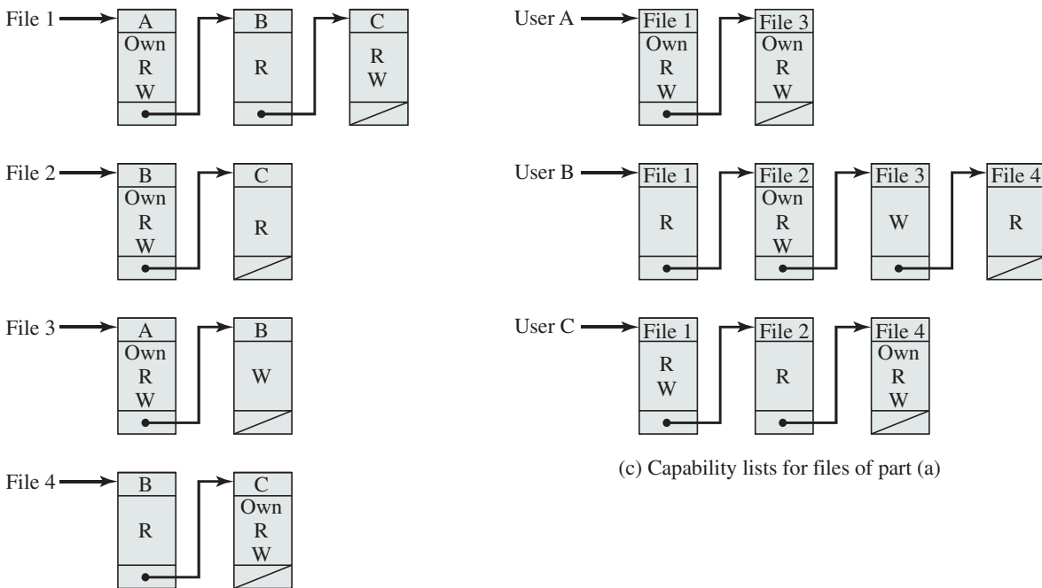
(b) Access control lists for files of part (a) Figure 12.15 Example of Access Control Structures
