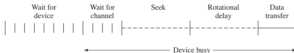
Figure 11.6 Timing of a Disk I/O Transfer
