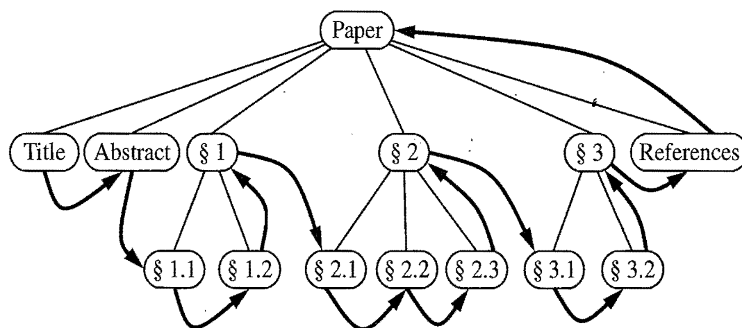
Figure 7.8: Postorder traversal of the ordered tree of Figure 7.6.
