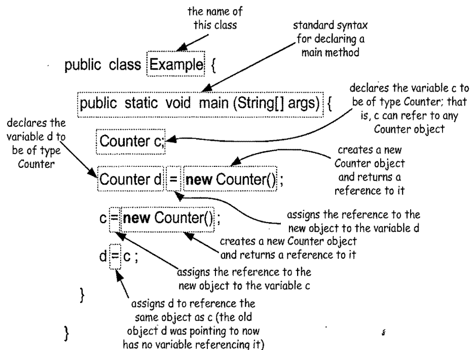
Figure 1.3: Example uses of the new operator.
