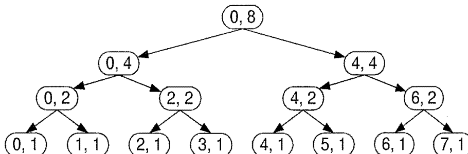
Figure 3.25: Recursion trace for the execution of BinarySum(0, 8) .
