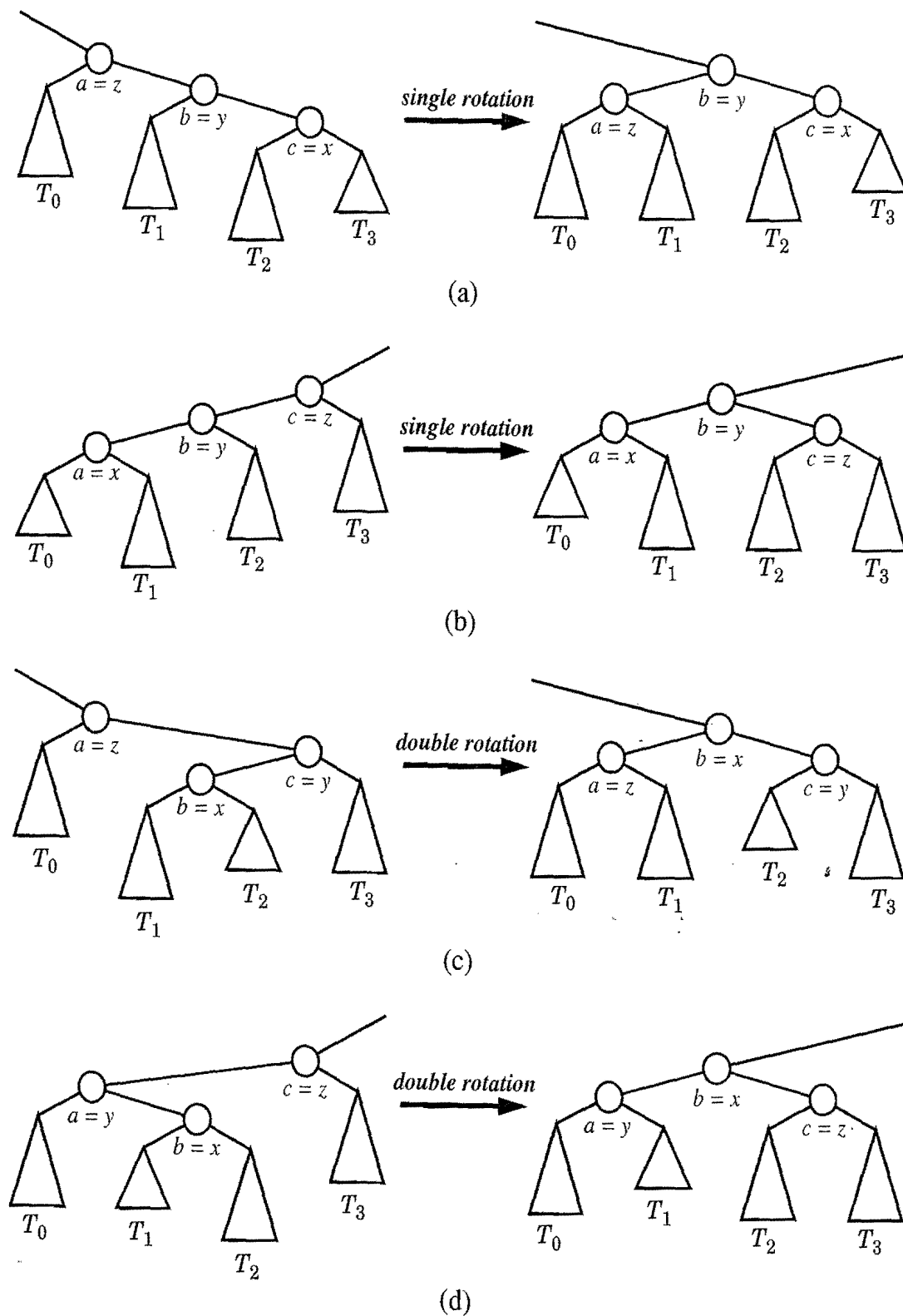
Figure 10.9: Schematic illustration of a trinode restructuring operation (Code Fragment 10.6): (a) and (b) a single rotation; (c) and (d) a double rotation.
