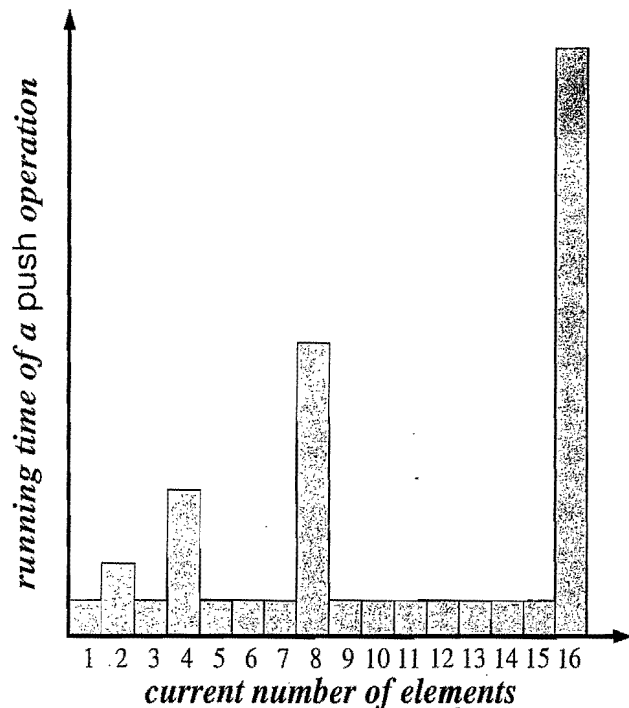
Figure 6.3: Running times of a series of push operations on a java.util.ArrayList of initial size 1.
