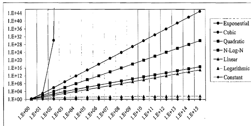
Figure 4.2: Growth rates for the seven fundamental functions used in algorithm analysis. We use base a = 2 for the exponential function. The functions are plotted in a log-log chart, to compare the growth rates primarily as slopes. Even so, the exponential function grows too fast to display all its values on the chart. Also, we use the scientific notation for numbers, where, aE+b denotes a10^b .
