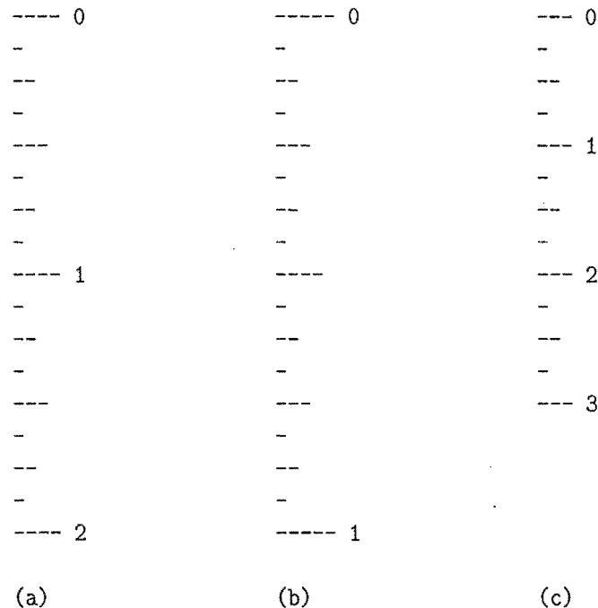
Figure 3.22: Three sample outputs of an English ruler drawing: (a) a 2-inch ruler with major tick length 4; (b) a 1-inch ruler with major tick length 5; (c) a 3-inch ruler with major tick length 3.
