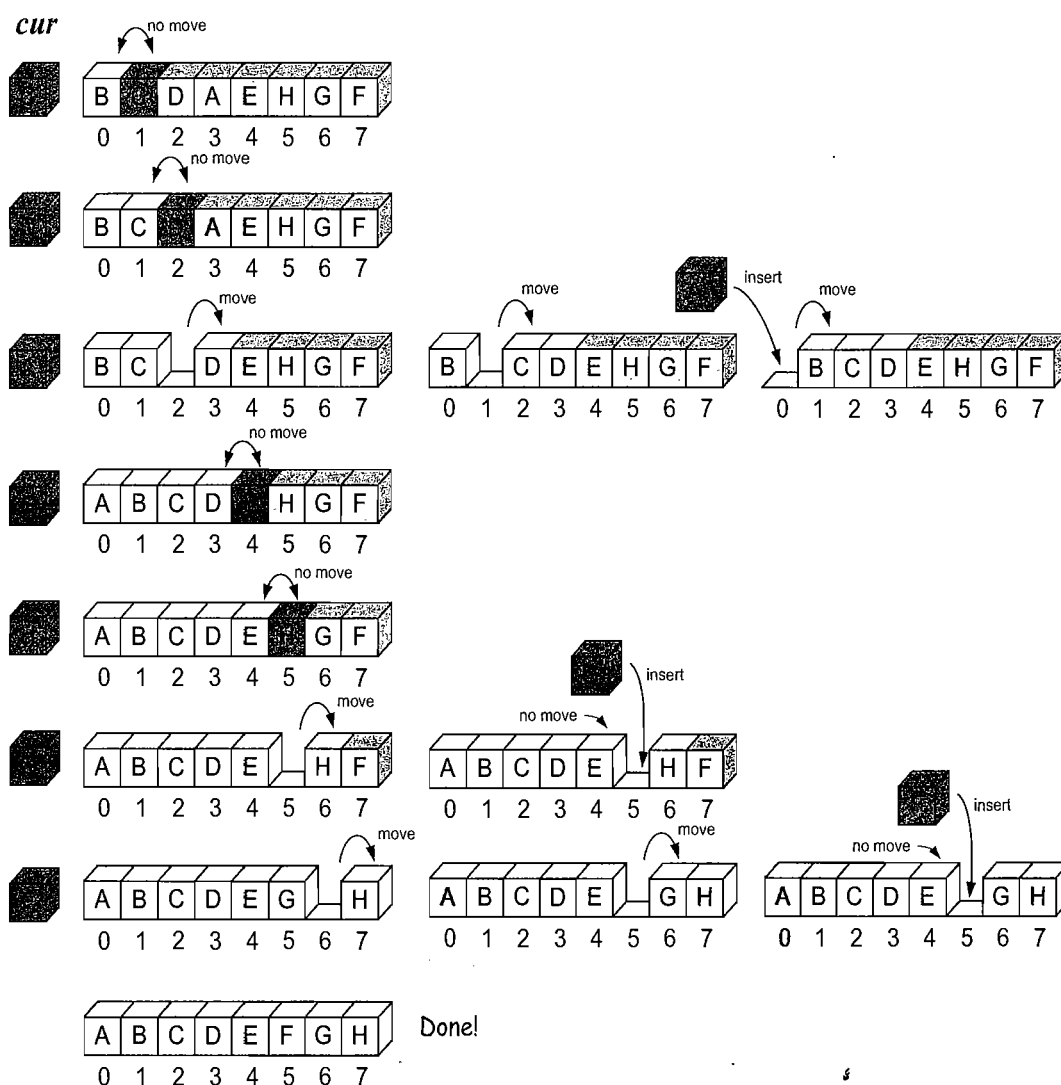
Figure 3.5: Execution of the insertion-sort algorithm on an array of eight characters. We show the completed (sorted) part of the array in white, and we color the next element that is being inserted into the sorted part of the array with light blue. We also highlight that character on the left, since it is stored in the cur variable. Each row corresponds to an iteration of the outer loop, and each copy of the array in a row corresponds to an iteration of the inner loop. Each comparison is shown with an arc. In addition, we indicate whether that comparison resulted in a move or not.
