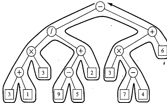
Figure 7.20: Euler tour traversal of a binary tree.
