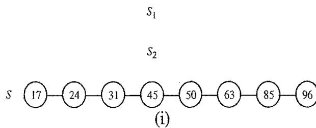
Figure 11.6: Example of an execution of the algorithm merge shown in Code Fragment 11.2.
