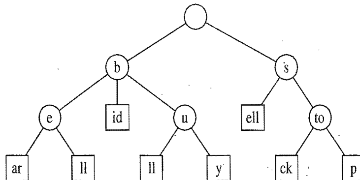
Figure 12.11: Compressed trie for the strings {bear, bell, bid, bull, buy, sell, stock, stop}. Compare this with the standard trie shown in Figure 12.9.
