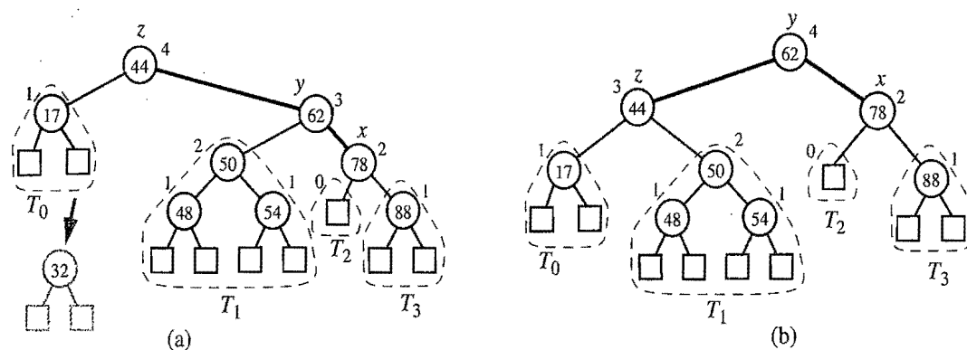
Figure 10.10: Removal of the entry with key 32 from the AVL tree of Figure 10.7: (a) after removing the node storing key 32, the root becomes unbalanced; (b) a (single) rotation restores the height-balance property.
