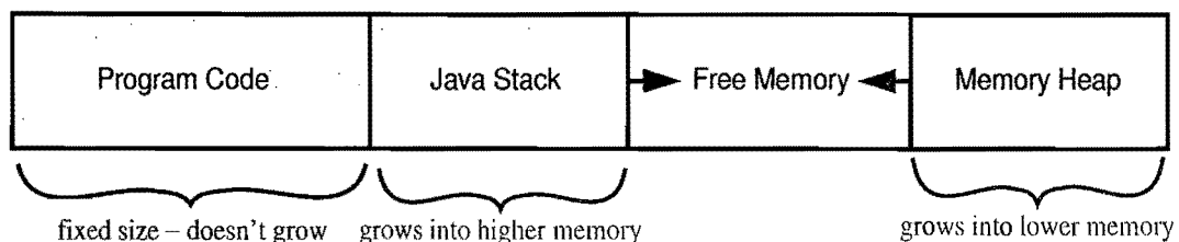
Figure 14.2: A schematic view of the layout of memory addresses in the Java Virtual Machine.
