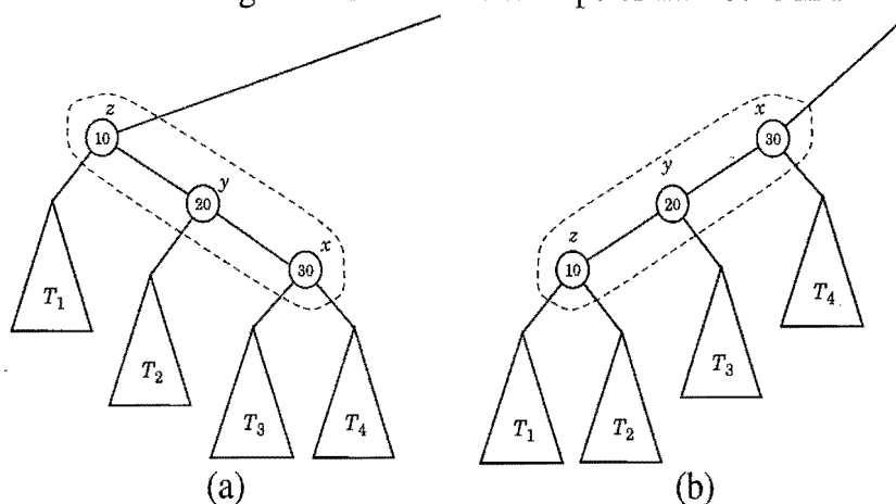
Figure 10.12: Zig-zig: (a) before; (b) after. There is another symmetric configuration where x and y are left children.
