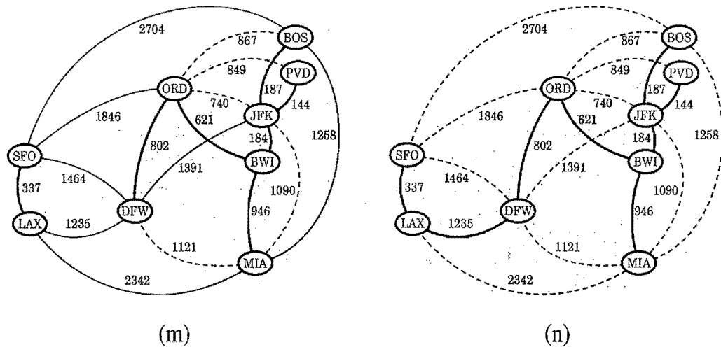
Figure 13.20: Example of an execution of Kruskal's MST algorithm (continued). The edge considered in (n) merges the last two clusters, which concludes this execution of Kruskal's algorithm. (Continued from Figure 13.19.)
