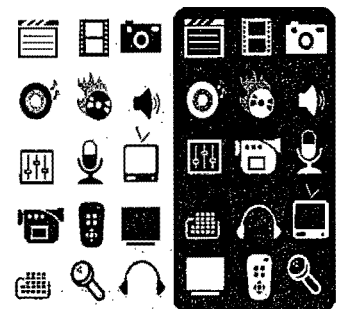
Modularity
