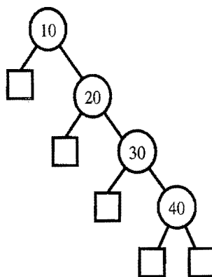
Figure 10.6: Example of a binary search tree with linear height, obtained by inserting entries with keys in increasing order.
