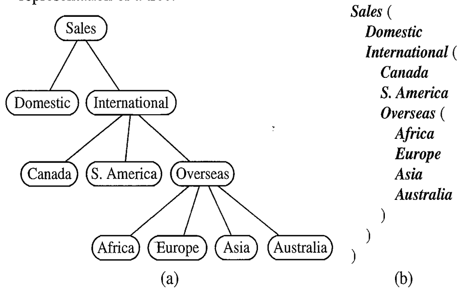
Figure 7.21: (a) Tree T ; (b) indented parenthetic representation of T .
