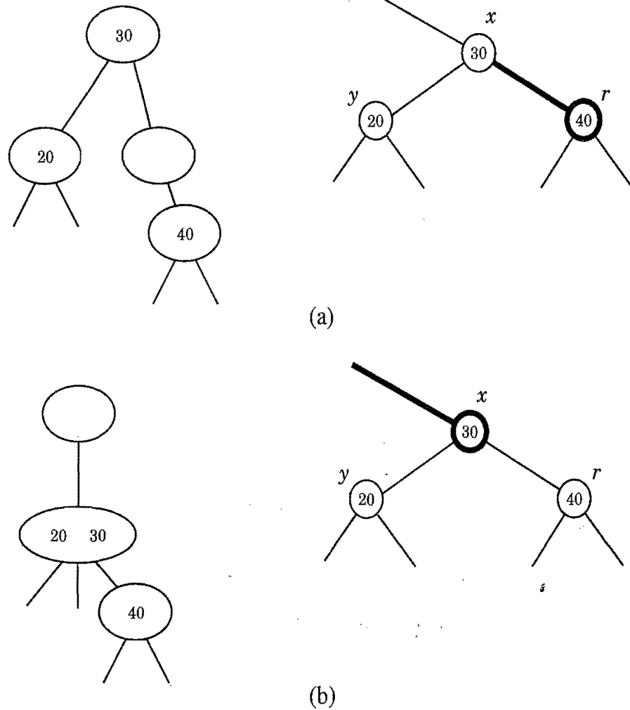
Figure 10.34: Recoloring of a red-black tree that propagates the double black problem: (a) configuration before the recoloring and corresponding nodes in the associated (2,4) tree before the fusion (other similar configurations are possible); (b) configuration after the recoloring and corresponding nodes in the associated (2,4) tree after the fusion.
