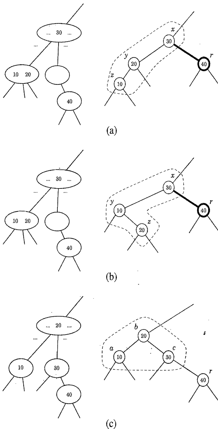
Figure 10.32: Restructuring of a red-black tree to remedy the double black problem: (a) and (b) configurations before the restructuring, where r is a right child and the associated nodes in the corresponding (2,4) tree before the transfer (two other symmetric configurations where r is a left child are possible); (c) configuration after the restructuring and the associated nodes in the corresponding (2,4) tree after the transfer. The grey color for node x in parts (a) and (b) and for node b in part (c) denotes the fact that this node may be colored either red or black.
