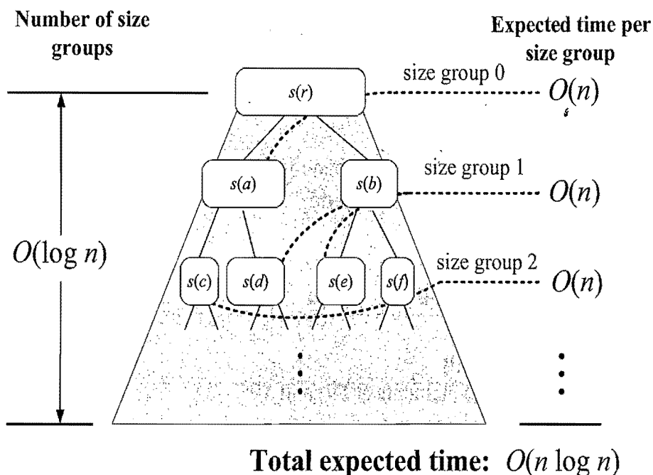
Figure 11.13: A visual time analysis of the quick-sort tree T . Each node is shown labeled with the size of its subproblem.
