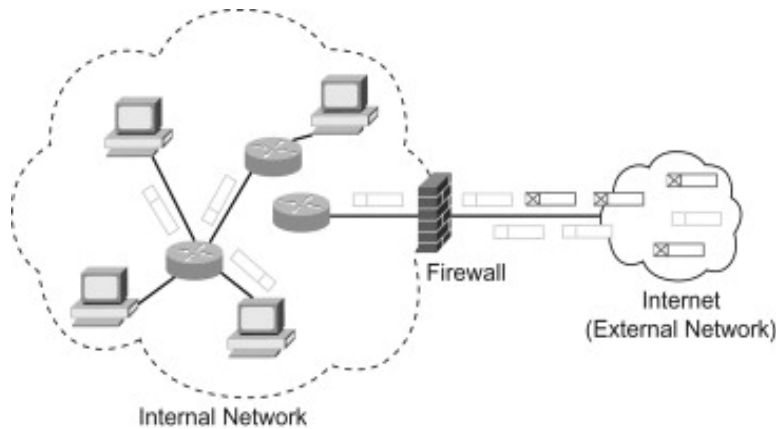
Fig. 3 Firewall setup
