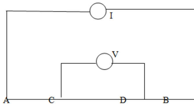
Fig 1: diagram of Schlumberger electrode Array
