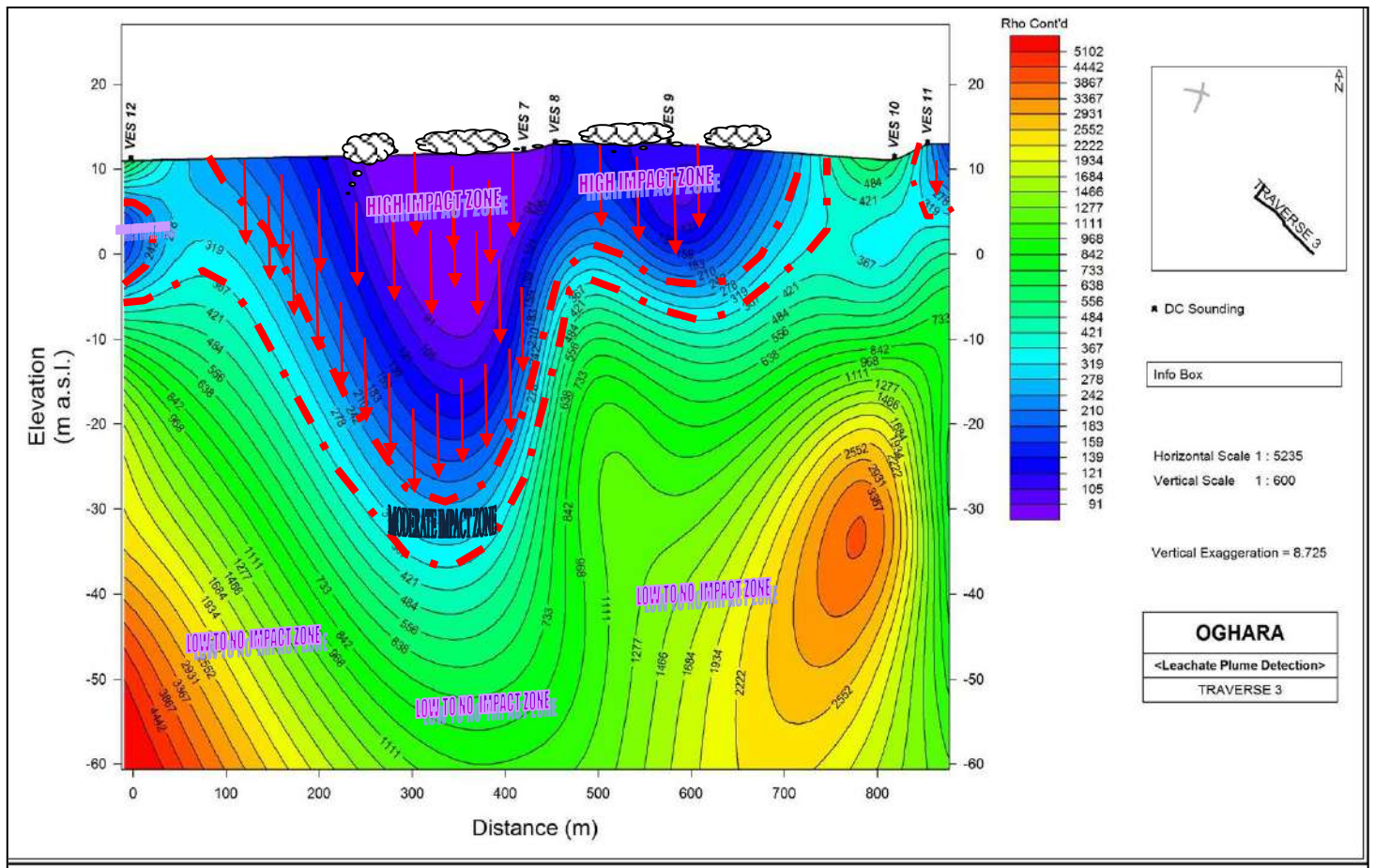
Fig. 8: The 2-D Section Beneath Profile 3
