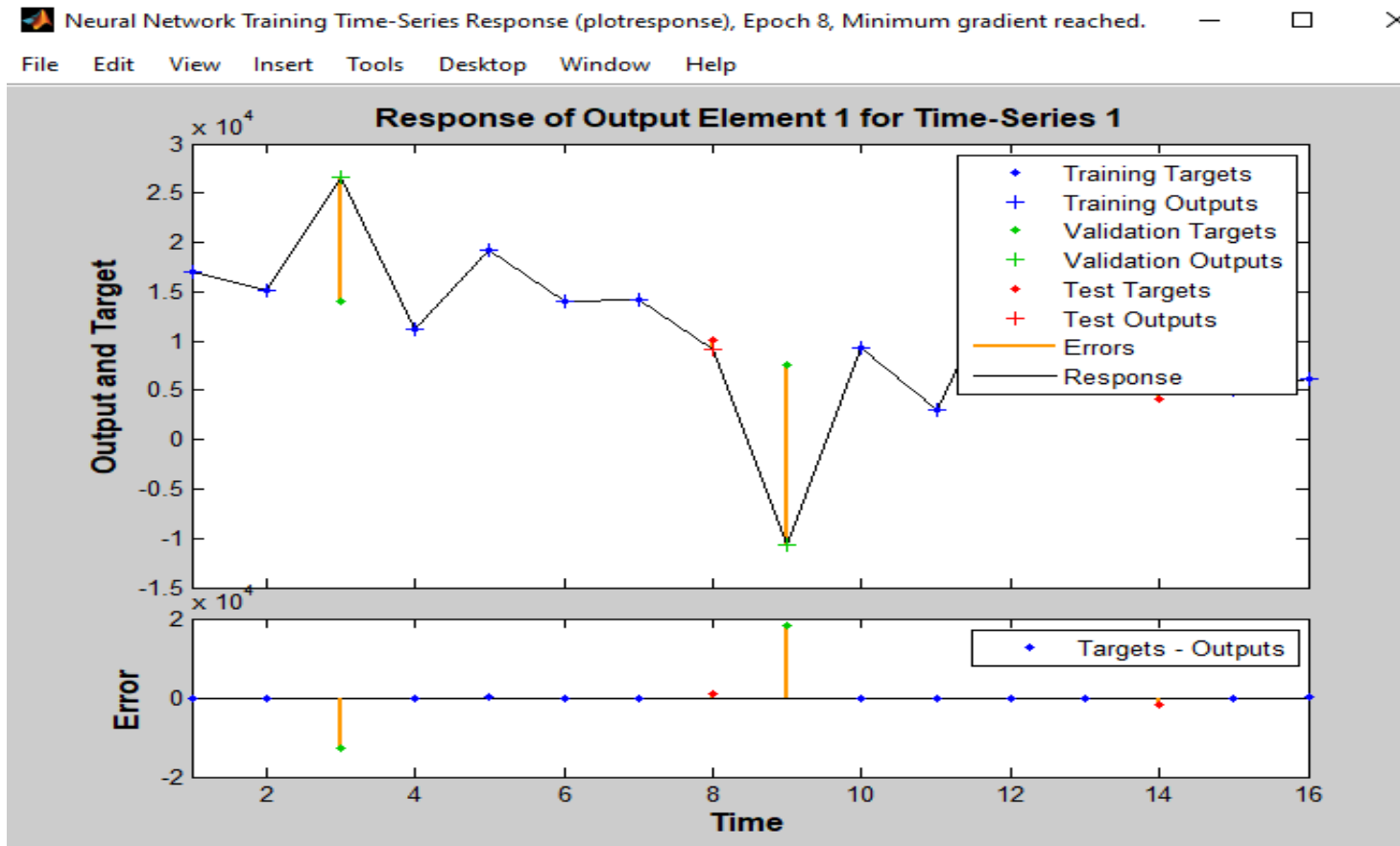
Fig. 7. Response of the Output variables and the Predicted Target
