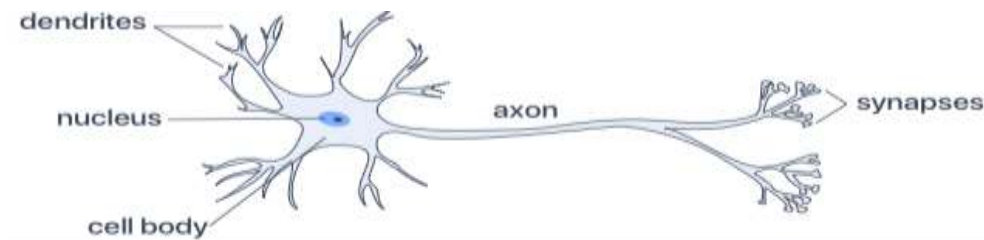
Fig. 1. Biological Neuron
