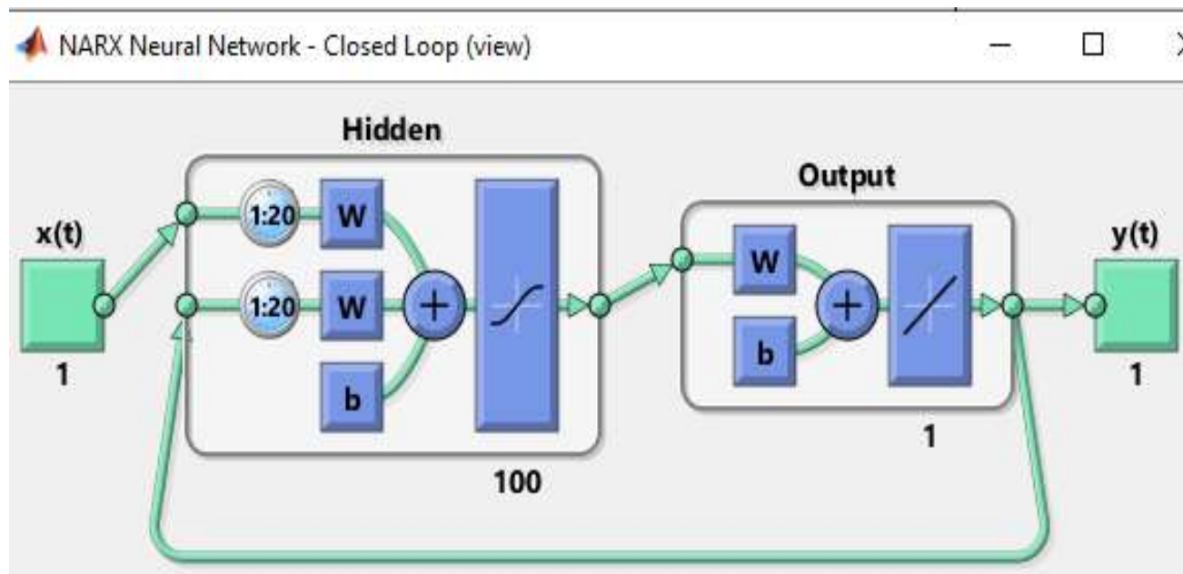
Fig. 8. Neural Networks Close Loop
