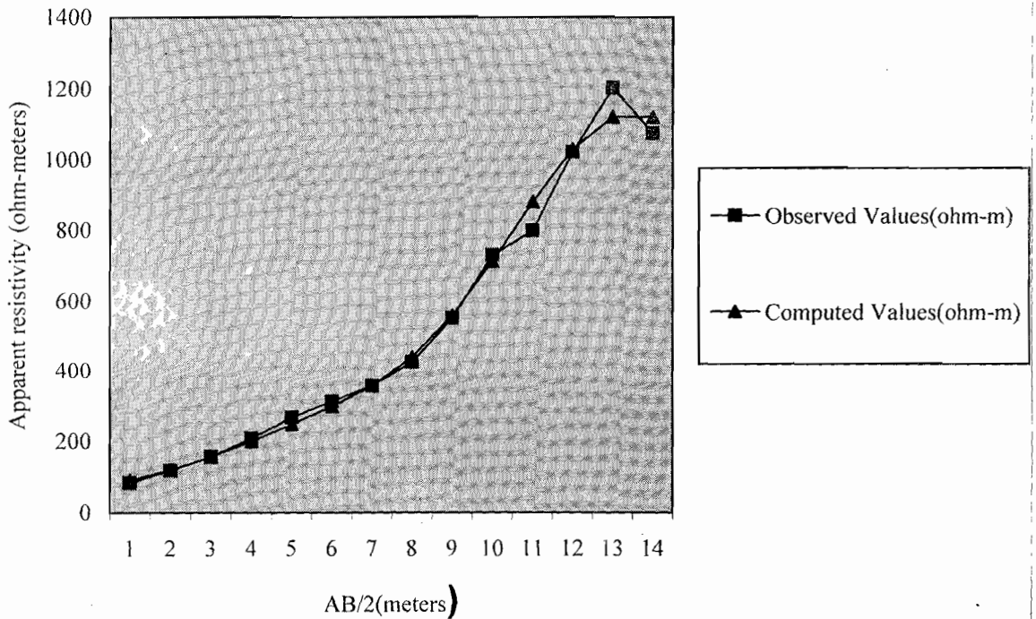
Figure 3: Afuze site - VES Number 3
