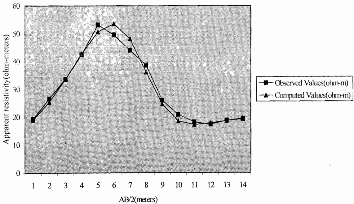
Figure 2: Afuze site - VES Number 2
