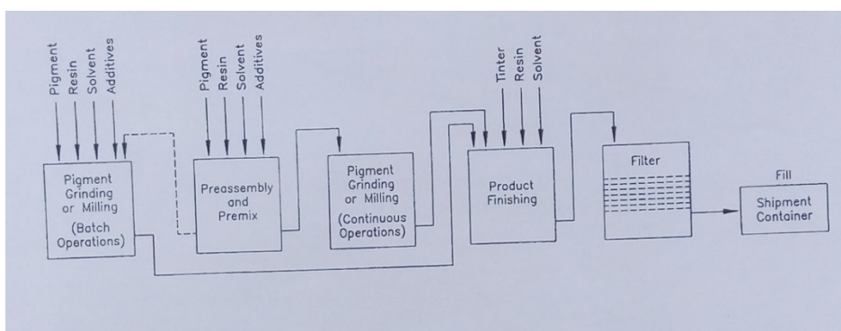
Fig. 3. Flow diagram of paint manufacturing process.
